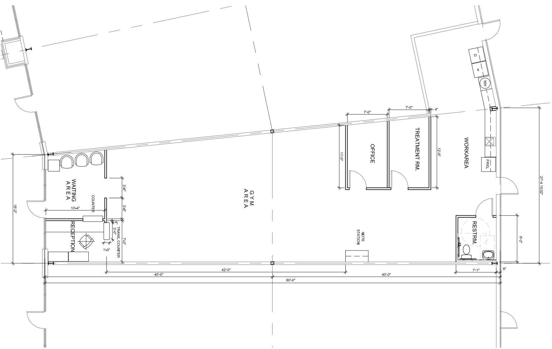
1 MAIN FLOOR PLAN
